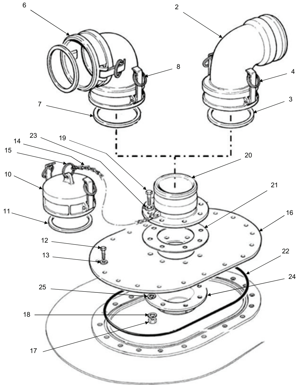
Figure 7. Filler/Discharge Assembly.
